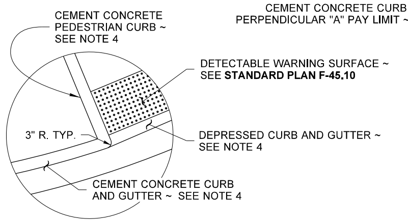
CURB RADIUS DETAIL B
