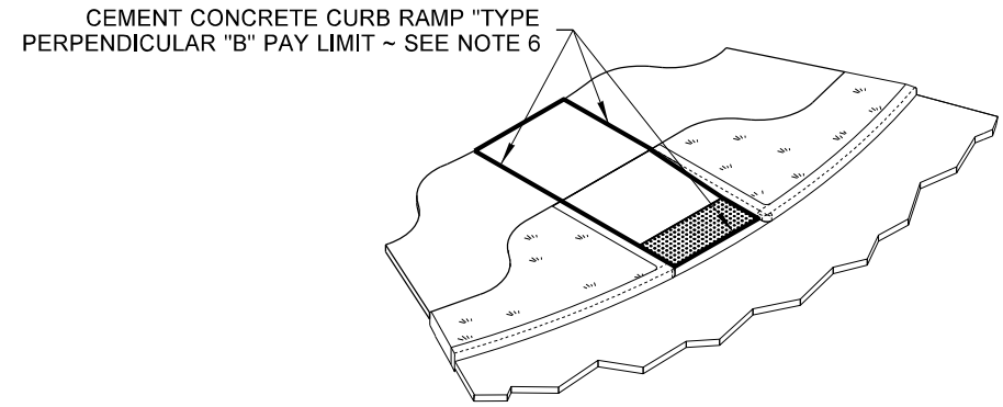
ISOMETRIC VIEW TYPE PERPENDICULAR B PAY LIMIT
