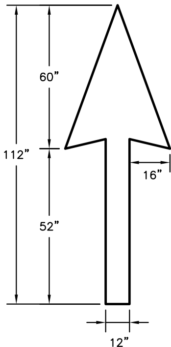
STRAIGHT ARROW
