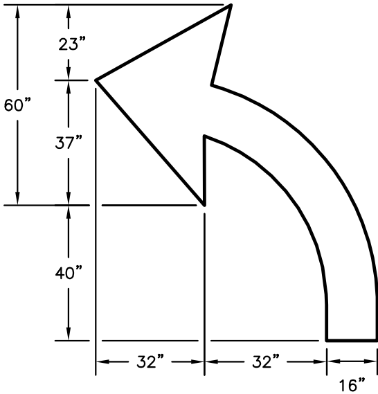
LEFT-TURN ARROW
