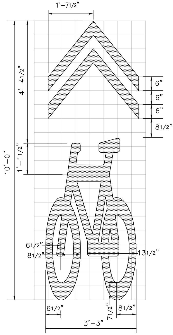
SHARROW SHARED LANE DETAIL
