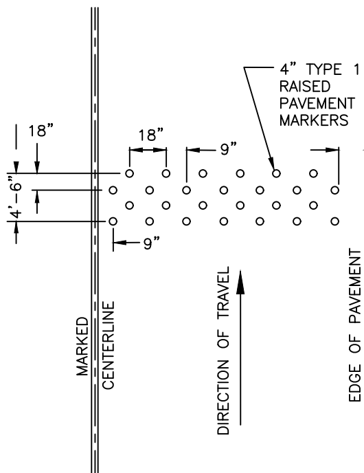
RUMBLE STRIP
