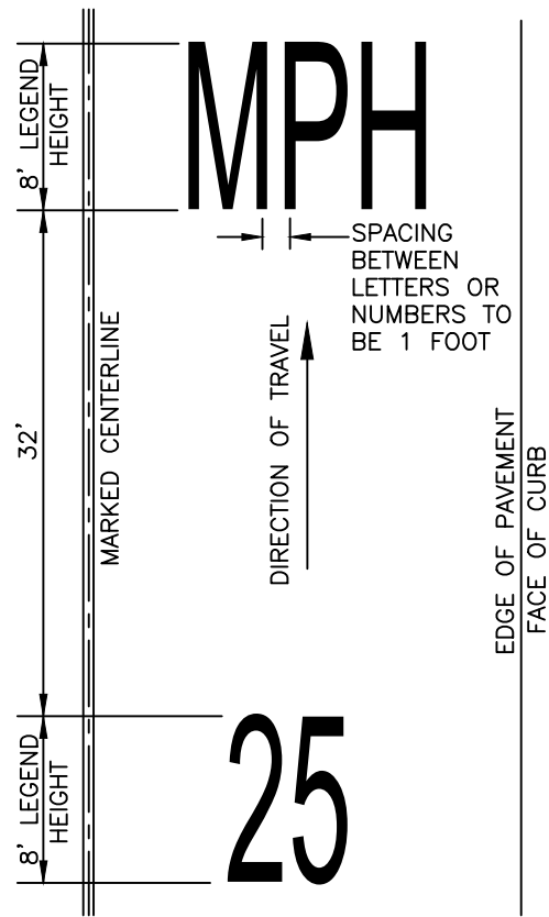
25 MPH LEGEND
