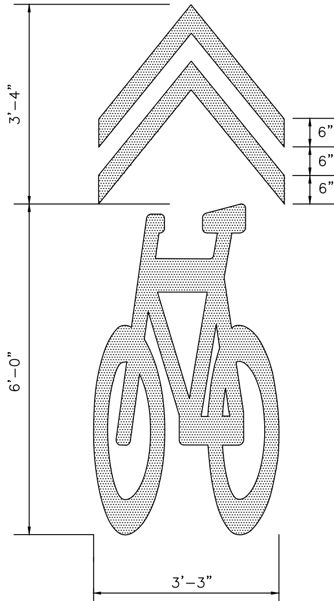
SHARROW SHARED LANE DETAIL
