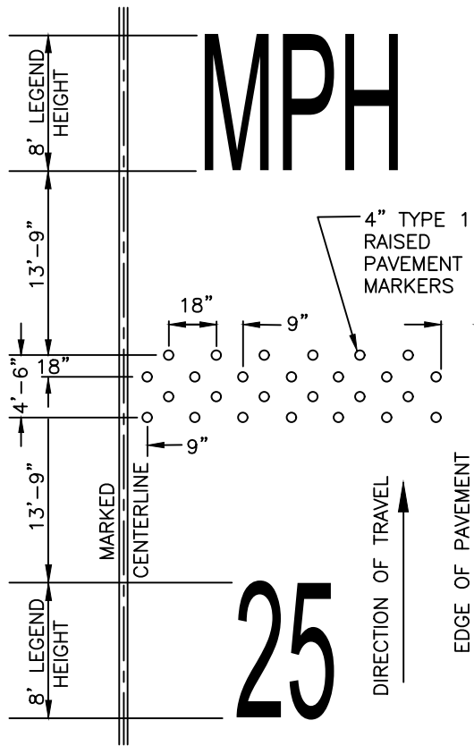
RUMBLE STRIP W/25MPH LEGEND
